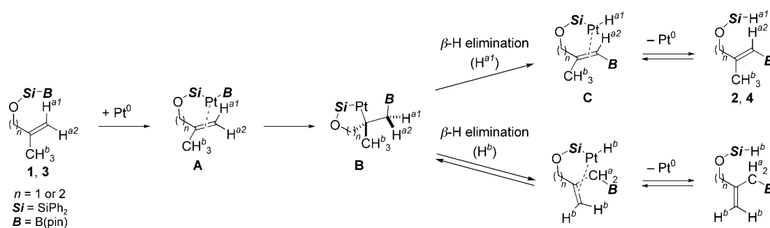
Scheme 2. Possible reaction mechanism.
